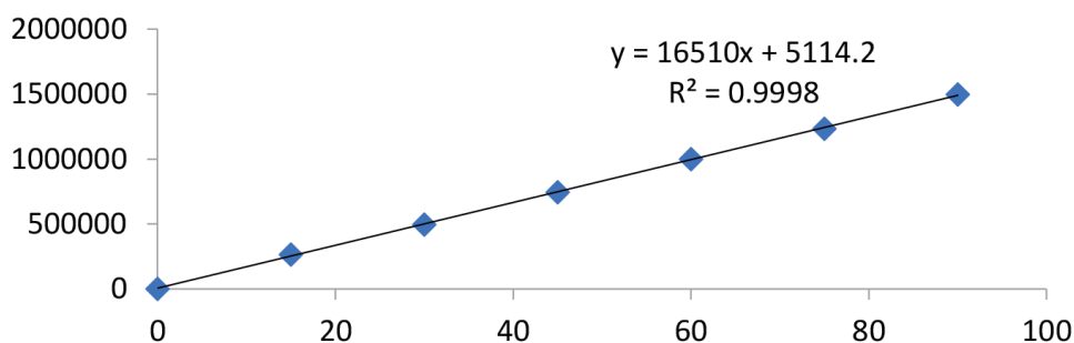
Figure 2: Calibration Curve of Linearity
